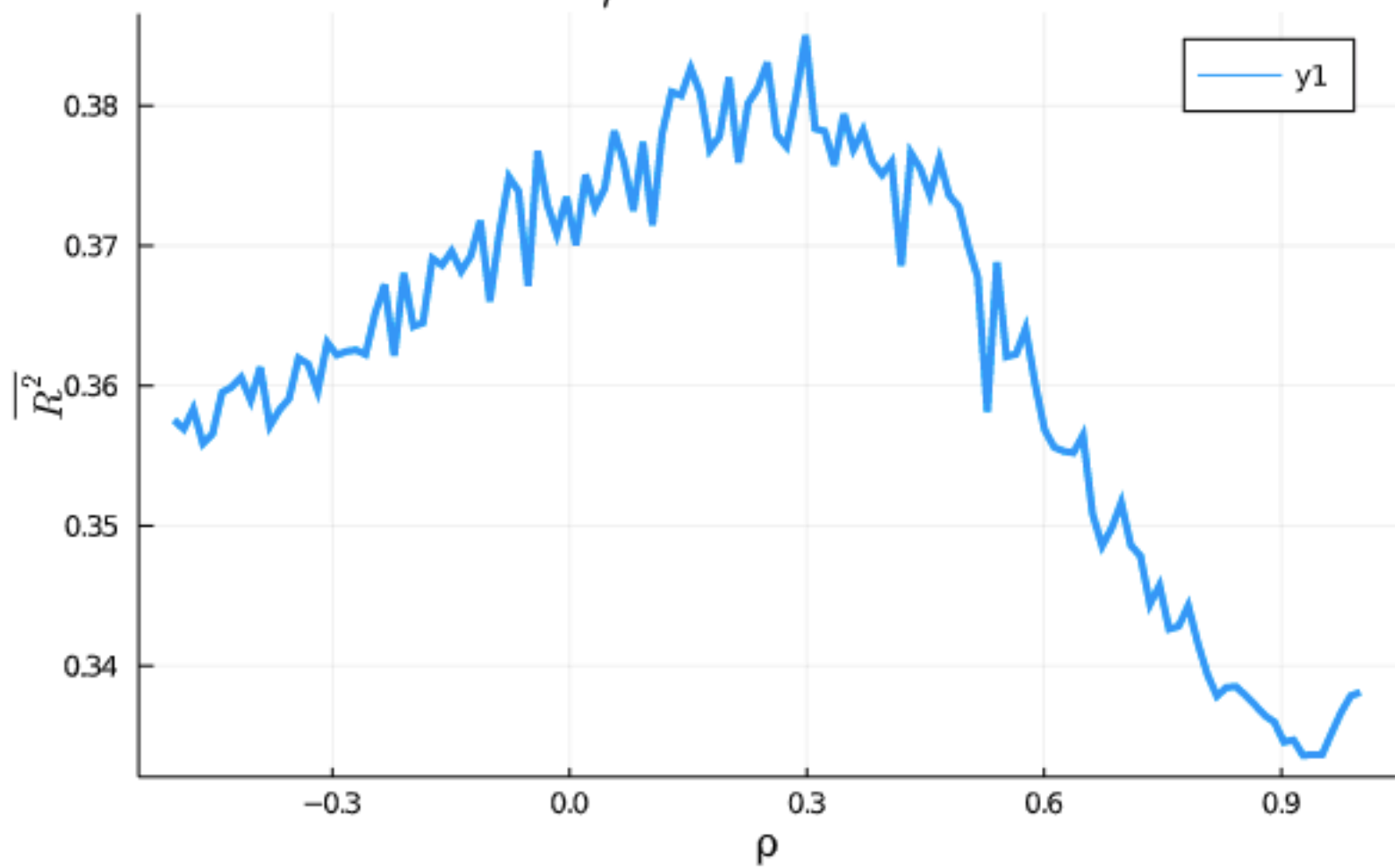
\overline{R}^2 vs. \rho for 3-Oscillator Grid
